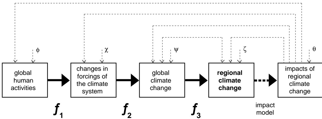
Figure 4.1 A simplified framework for deriving regional climate change scenarios consistent with stipulated anthropogenic climate change. The f_i refer to the required steps; thick lines indicate the flow of information; thin lines are some possible but neglected feedbacks; \phi , \chi , \psi , \zeta , \theta are additional, not explicitly considered or unknown factors.
