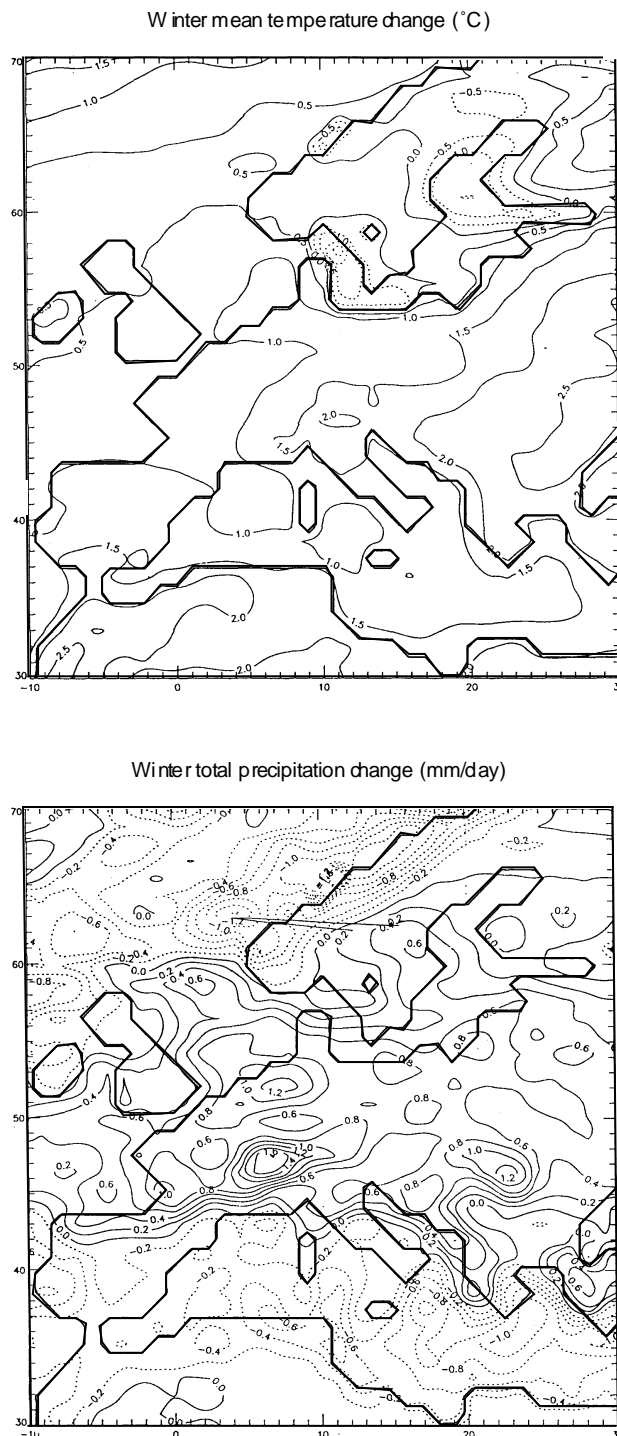
Figure 4.15 A Business as Usual climate change scenario for Europe by the year 2045 obtained from simulations with the ECHAM3-T106 high-resolution GCM. Shown are average changes from a five-year time window from the year 2045 relative to the means from a five-year control run. Boundary conditions for the two high-resolution GCM runs were taken from a control and a transient climate change simulation with the ECHAM1-T21/LSG-GCM (Cubasch et al. 1992), respectively. Temperatures are in °C, precipitation in mm/day. From Beniston et al. 1995.
