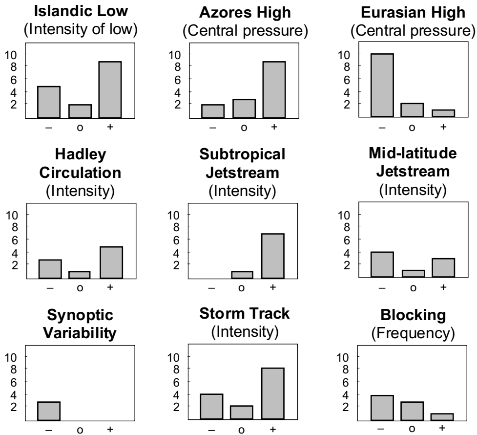
Fig. 1: Summary of changes in selected features of the atmospheric circulation in the North Atlantic/European sector, as simulated by different GCMs. Shown are the found numbers of studies for which the respective type of change was reported in the literature for the period 1975–1999. All data refer to the winter season and reflect the GCMs' response to a doubled CO 2 or time-dependent greenhouse-gas only forcing. The signs "-", "o", and "+" refer to a decrease, no change or increase of the respective feature's intensity or frequency. After Gyalistras (2000a).
