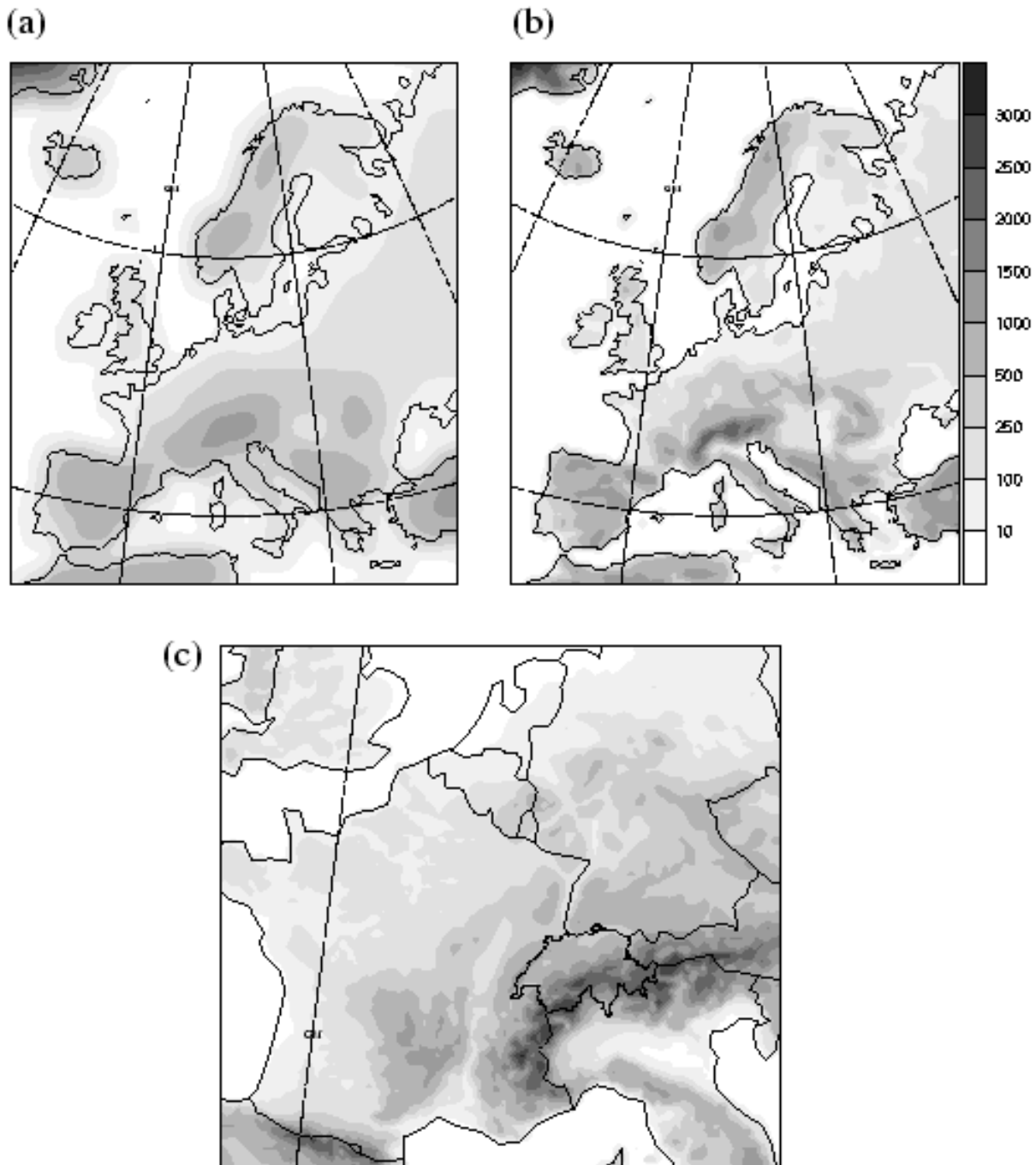
Figure 4.8 The European and Alpine orography for three spatial resolutions: (a) a typical coupled atmosphere-ocean climate GCM resolution (350 kilometers), (b) a typical meso-scale resolution (56 kilometers), and (c) a fine-mesh mesoscale resolution (14 kilometers).
