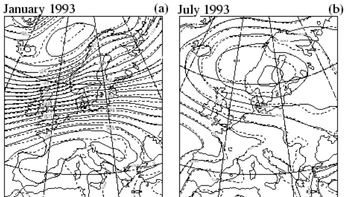
Figure 4.9 Simulated (full lines) and observed (dashed lines) mean sea level pressure for regional climate simulations of (a) January 1993 and (b) July 1993. After Cress et al. (1994).
